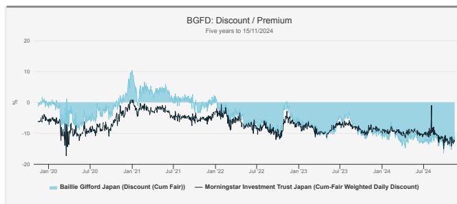
Fig.9: Discount
